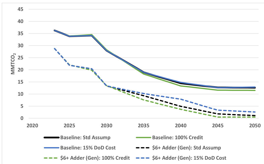
Figure F.64. Adder on Gen: Emissions from NC In-State Generation across Battery Assumptions
