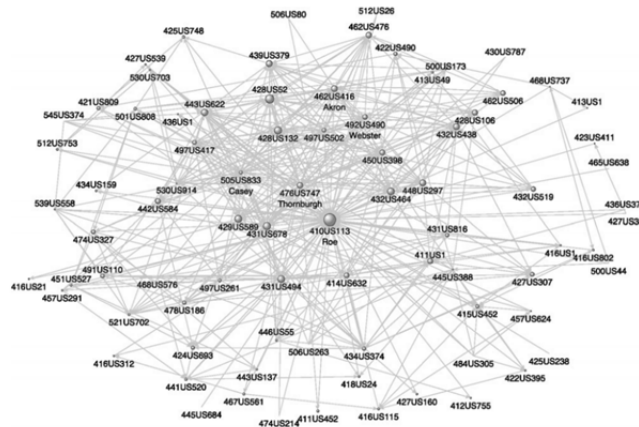
Figure 1: A visual of a network; this plot shows Roe v. Wade and its neighboring cases. Each dot represents a case and each gray arrow represents a citation from one case to another. 17
